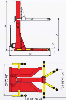
"Pallet jack" style device allows the lift to be moved wherever you need it.
