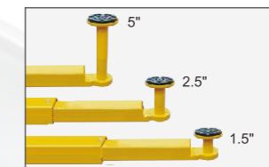
Standard drop-in adaptors 1.5", 2.5" & 5" extension high adaptors to fit different trucks and lifting height.
